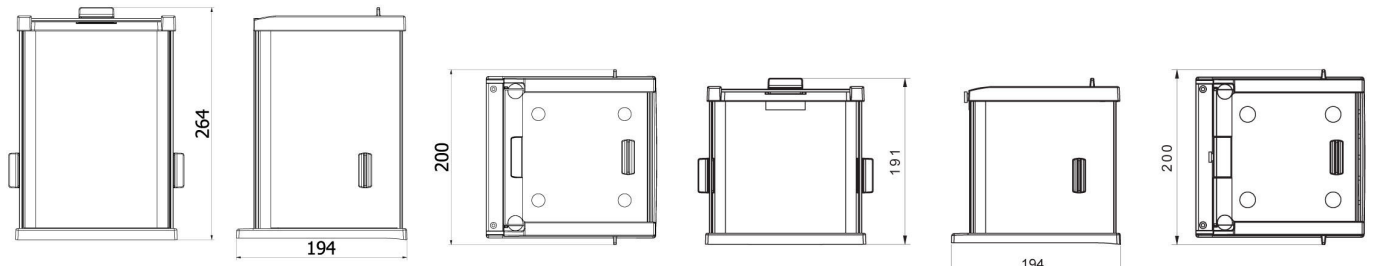
Anti-draft chamber for balances with 128x128 mm weighing pan
