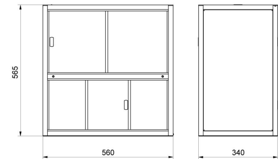
Anti-draft chamber for WAY-KO mass comparators
