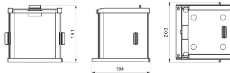
Anti-draft chamber for X2 and R2 precision balances
